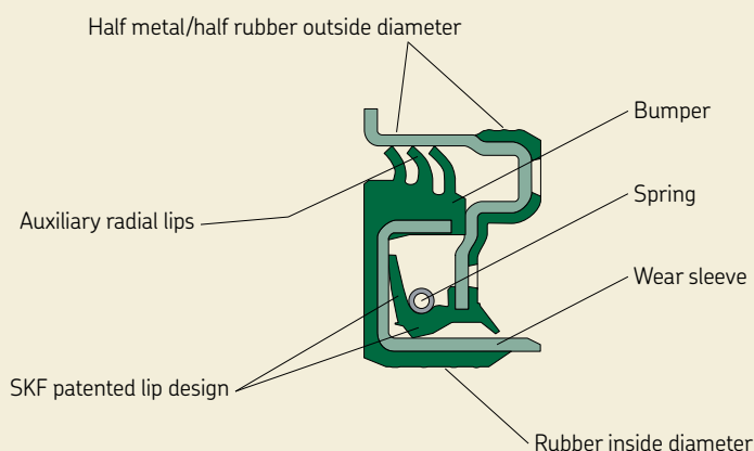
SKF Mudblock seal MUD7
