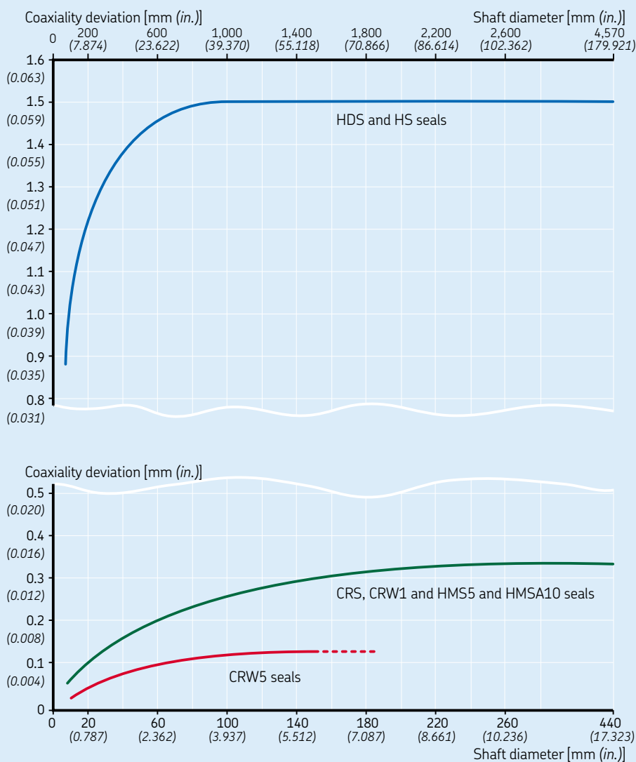
Maximum permissible deviation from coaxiality as a function of shaft diameter
