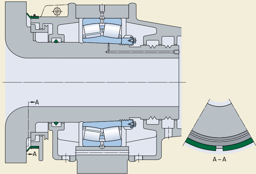
Sealing arrangement and installation
